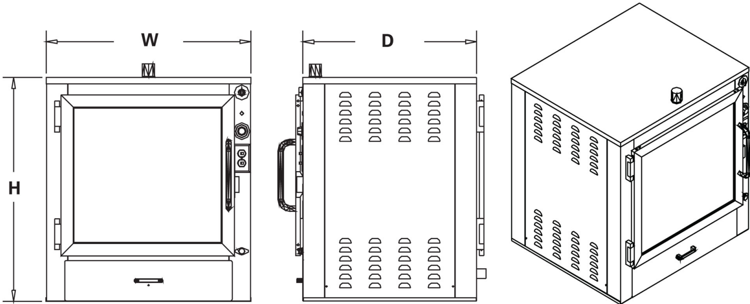
Interior Dimensions: 25-1/2" H x 26-1/2"W x 27-1/2" D (oven)
